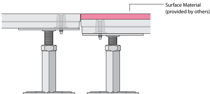
Transition Made Using Adjustable Head without Stringers
