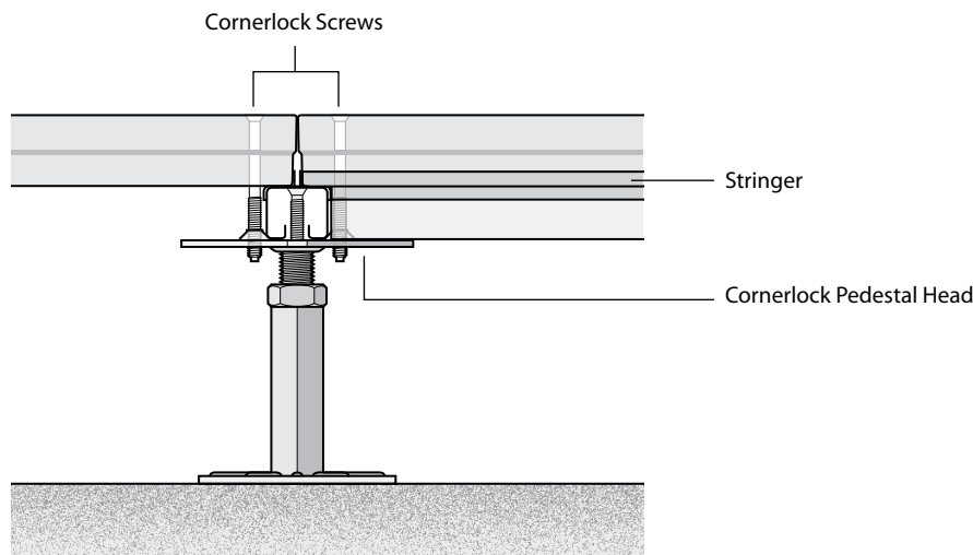
Transition from Cornerlock to Stringer-Supported Panels
