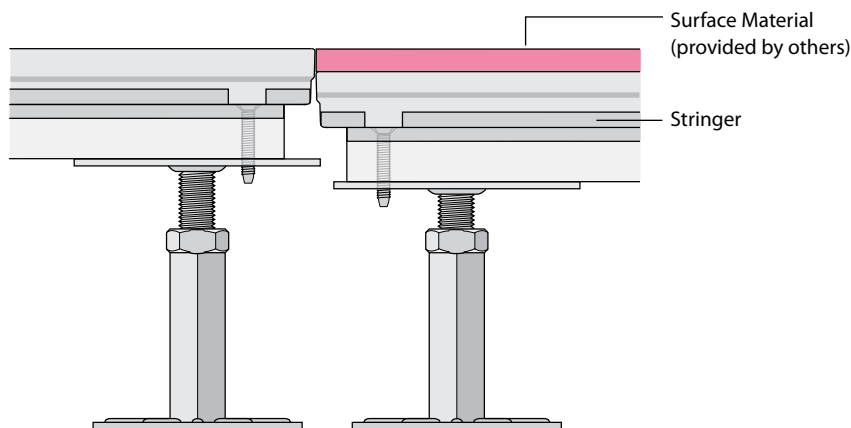
Transition Made Using Adjustable Head with Stringers
